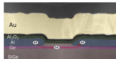
Fig.: Transmission Electron Micrograph of a Ge Josephson junction fabricated at the CEA clean room. (Courtesy of J. Labar, EK Budapest)
